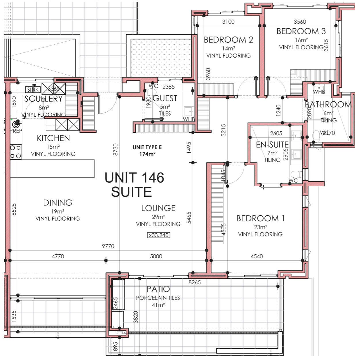
UNIT LAYOUT PLAN
