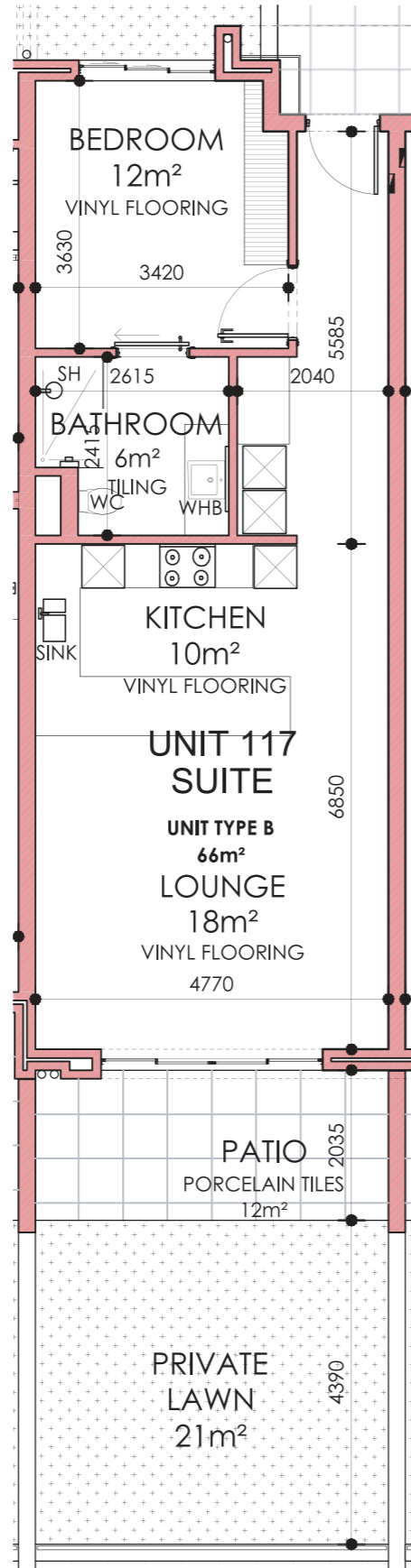
UNIT LAYOUT PLAN
