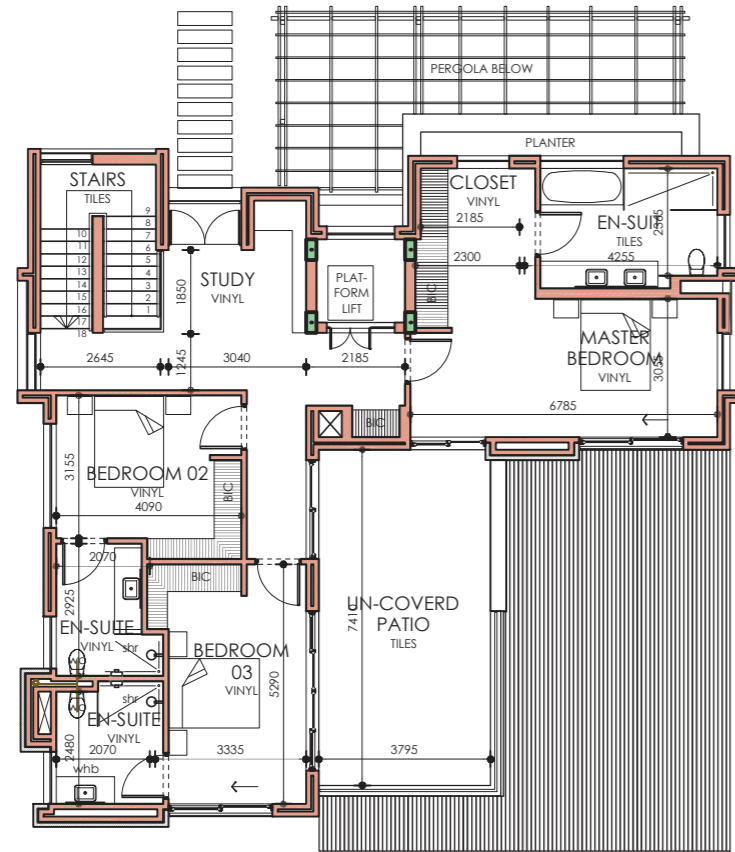
FIRST FLOOR UNIT LAYOUT PLAN
