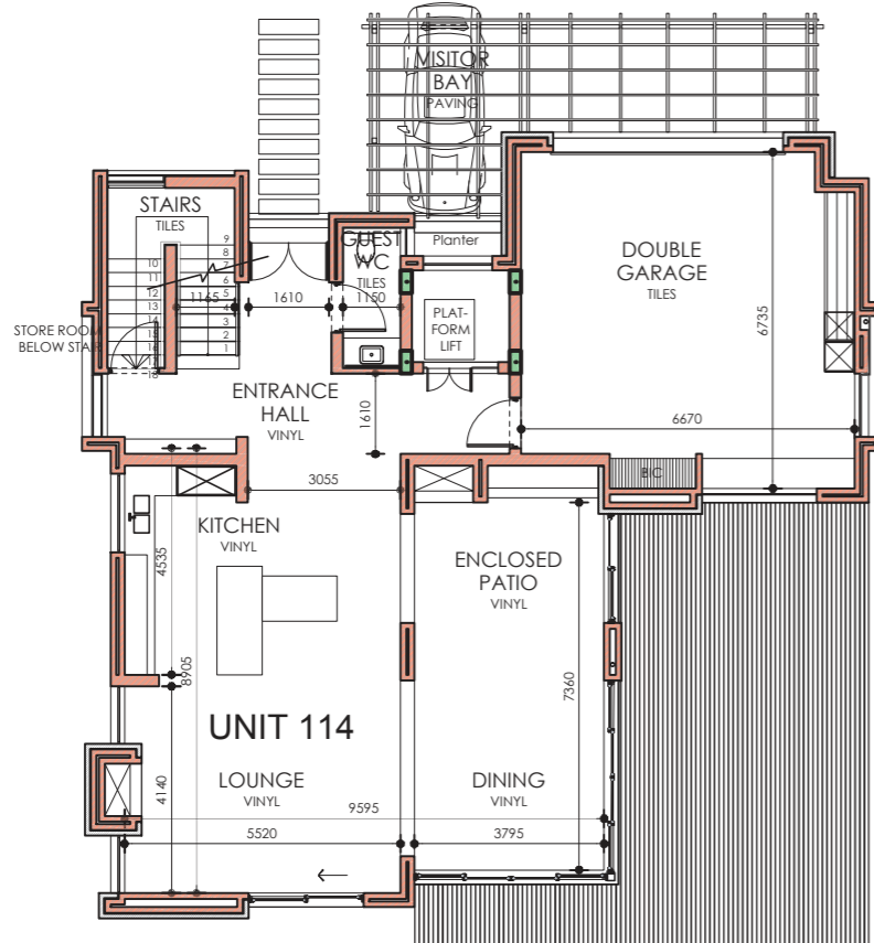
GROUND FLOOR UNIT LAYOUT PLAN
