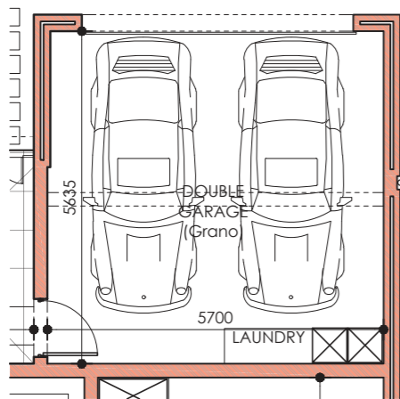
GARAGE ON GROUND FLOOR
