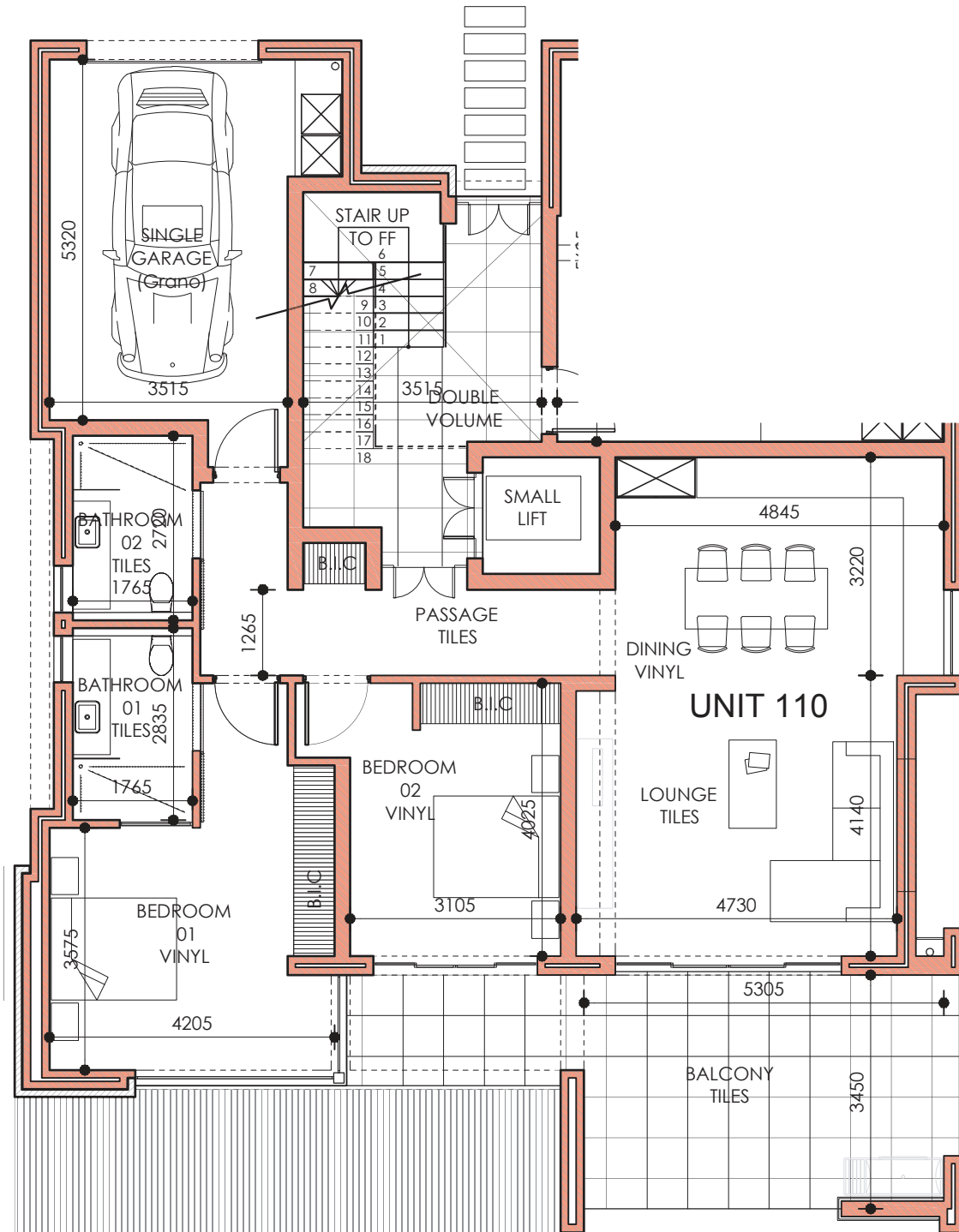
UNIT LAYOUT PLAN
